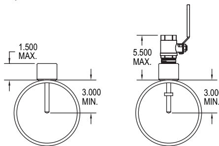
Figure 12: Stack height
