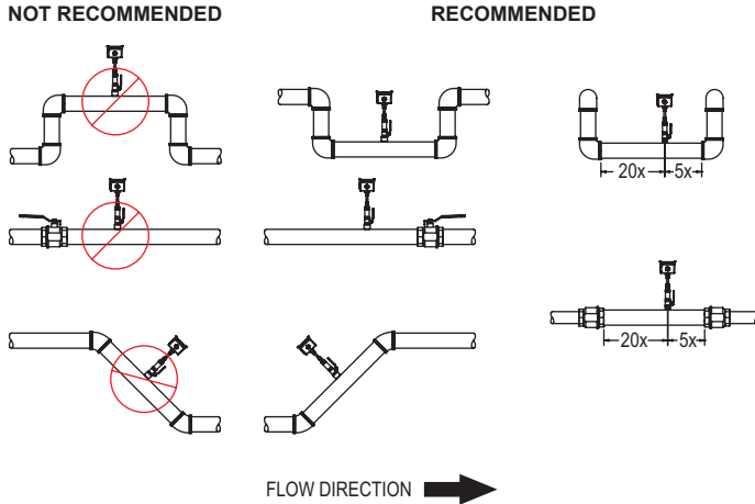
Figure 3: Proper installation location
