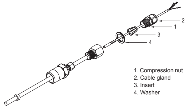
Figure 13: Thermowell assembly with PG gland
