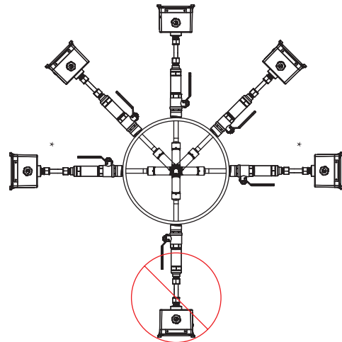
Figure 2: Proper installation orientation
